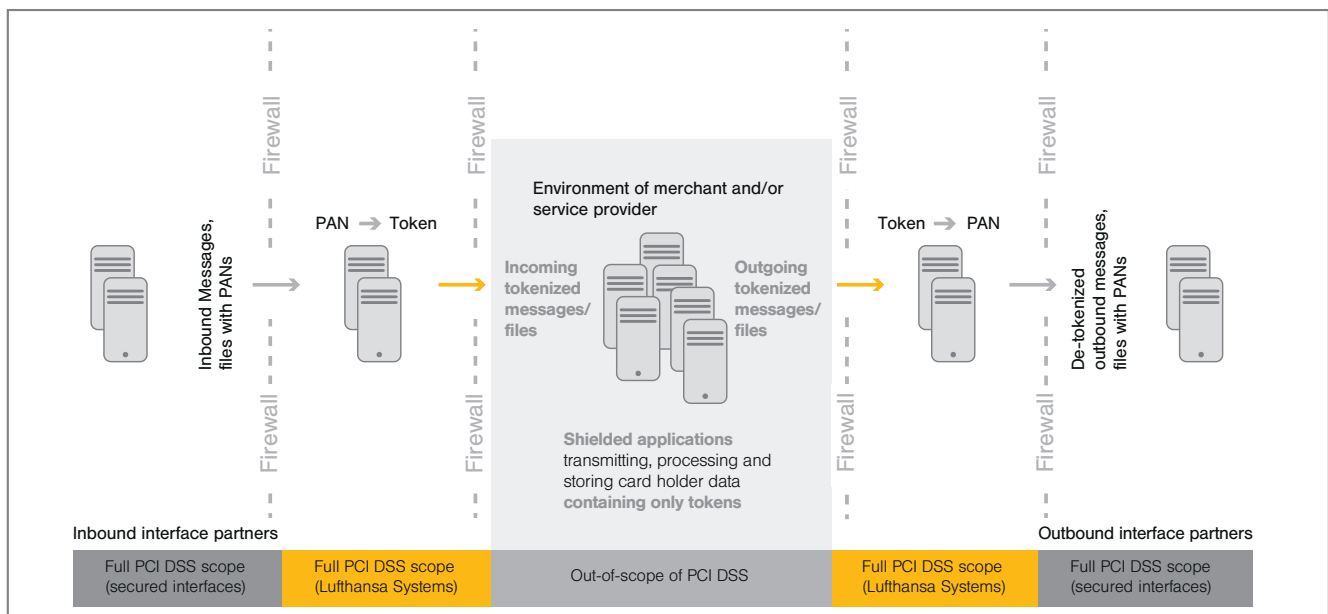
Data process flow with PCI Compliance Engine: applications and networks of merchants and service providers are out-of-scope of PCI DSS.
